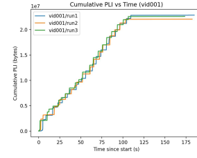
Fig. 3. PLI - Time graph for one of 10 videos showing that highly identical slopes between three runs. PLI - Time Graph of others is publicly available on our github repository [3].
