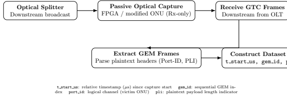
Fig. 2. Attacker-side observation pipeline: passive optical capture under the same splitter enables reception of downstream GTC frames, extraction of GEM frames, and construction of a PLI-based dataset ( gems.csv ).
